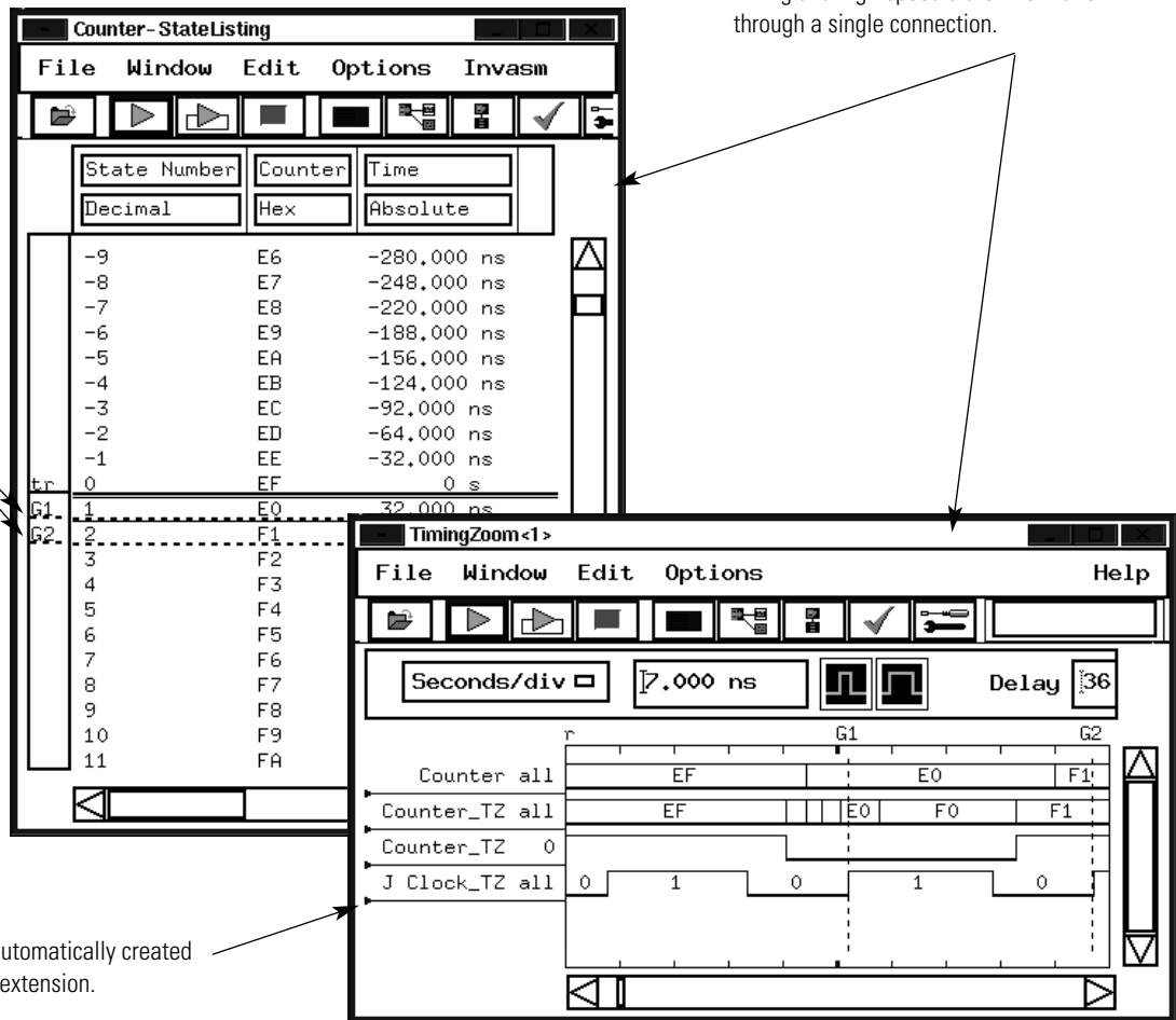
Figure 4.3. Verifying critical edge timing in your system is easy with Agilent Technologies' 2 GHz Timing Zoom technology.
