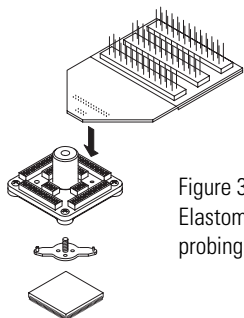
Figure 3.5. Agilent Wedge Probe Adapters for QFP package
