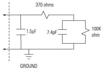
Figure 6.10. Equivalent probe load for the Agilent 16557D, 16710A, 16711A and 16712A, general-purpose lead set.
