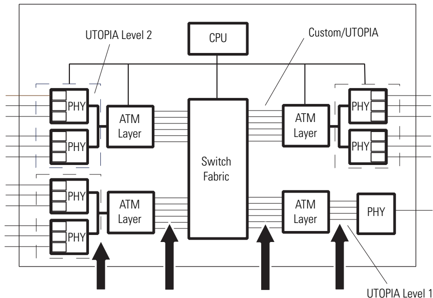
Figure 5.5. Typical ATM Switch Design.
