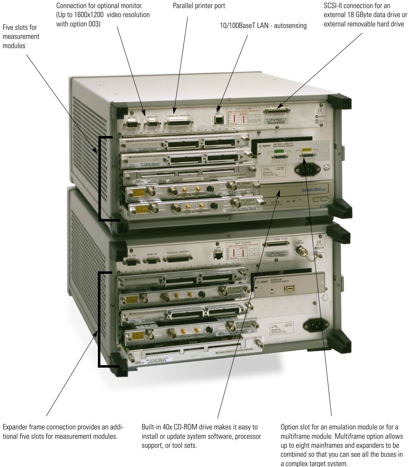
Figure 2.2. The mainframe and expander frame provide advanced capabilities for debugging complex target systems.
