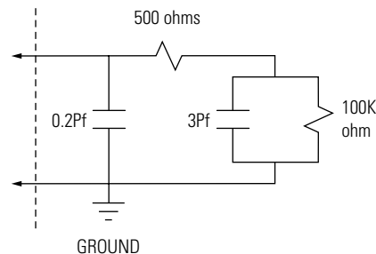
Figure 6.11. Equivalent probe load for the Agilent 16517A/18A.
